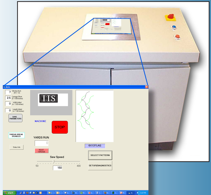
Full replacement enclosure with touchscreen and operator controls
