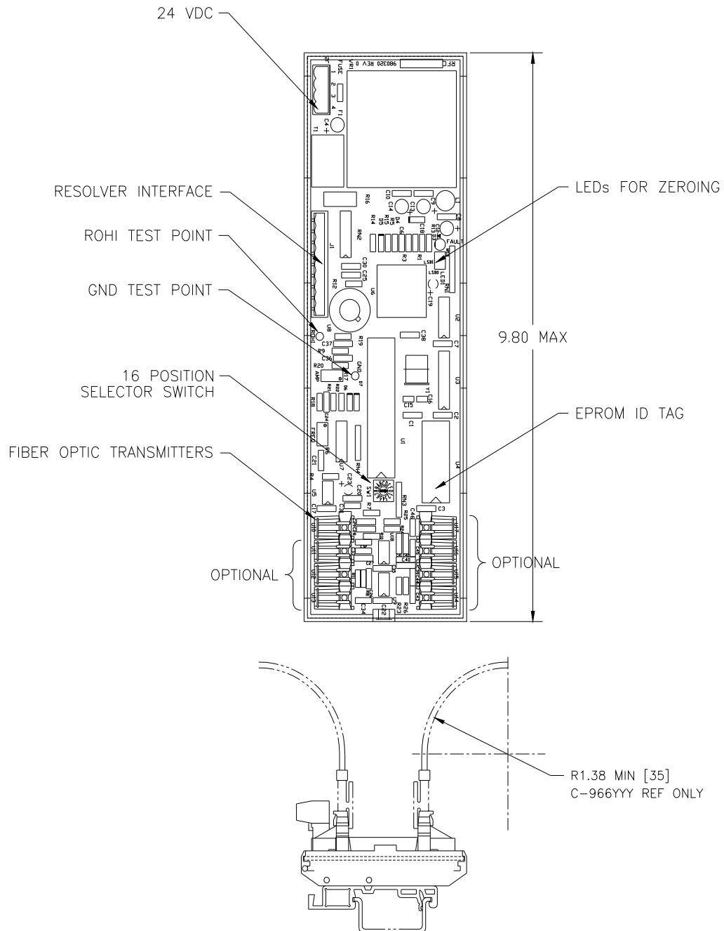
Figure 2 - RFC-240X Layout
