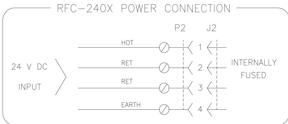
Figure 3 - Connection Interconnection
